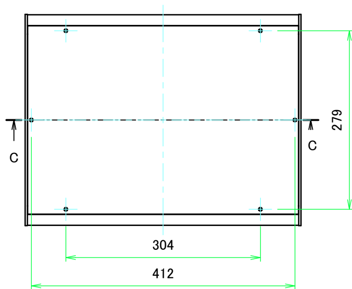
E view
